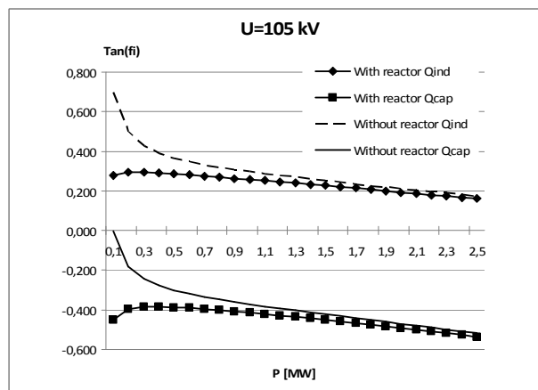
Fig. 5. \tan(\phi) in PCC as the function of power of WPP for overhead line (voltage 105 kV)
