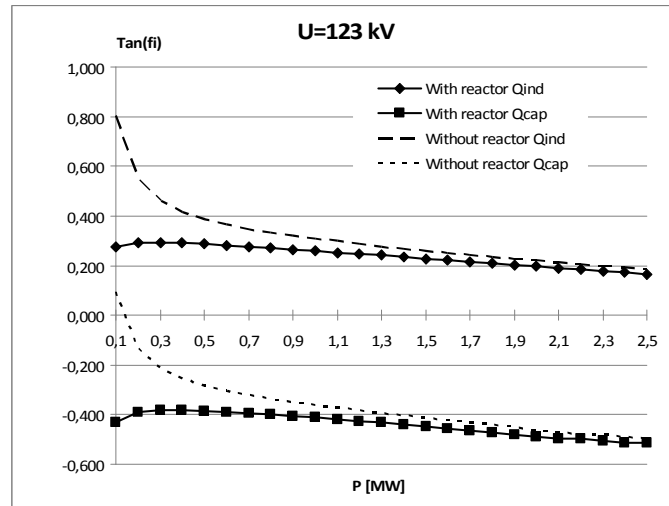
Fig. 6. \tan(\varphi) in PCC as the function of power of WPP for overhead line (voltage 123 kV)
