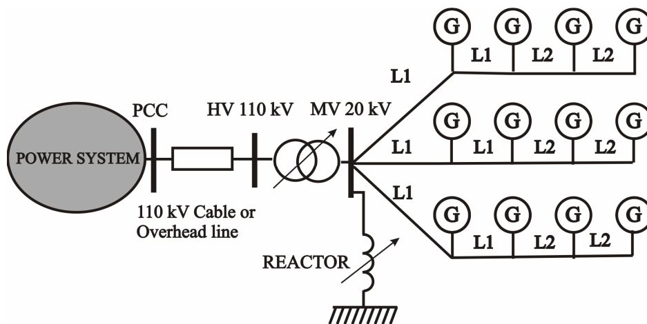
Fig. 2. Electric diagram of 30 MW WPF
