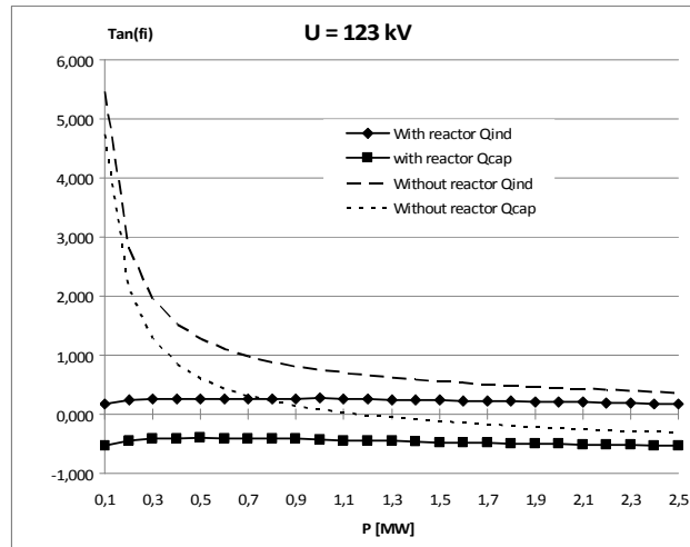
Fig. 4. \tan(\phi) in PCC as the function of power of WPP for cable line (voltage 123 kV)
