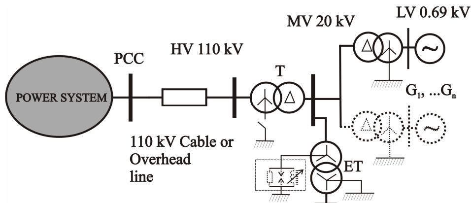
Fig. 1. Connection of typical WPF to power system
