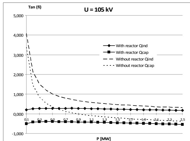
Fig. 3. \tan(\varphi) in PCC as the function of power of WPP for cable line (voltage 105 kV)
