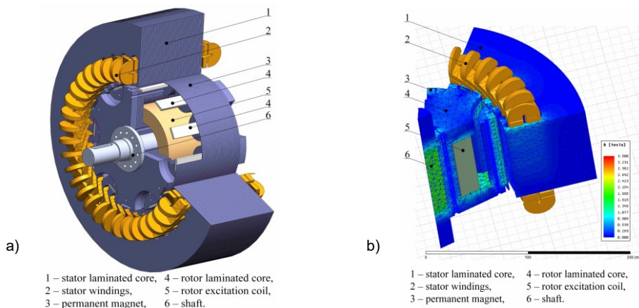
Fig.1. Design of the claw pole machine: a) visualization, b) model FEM.
