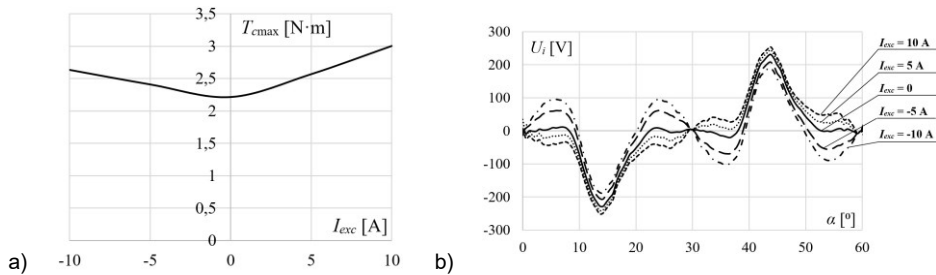
Fig.2. Test results of the machine: a) maximum cogging torque value, b) back-EMF waveforms.
